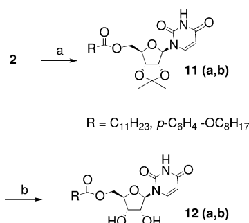
SCHEME 4 a) Py, lauroyl chloride ( 11a ), p -octyloxybenzoylchloride ( 11b ), room temperature, 24 hours; b) HCl (10%), room temperature, 12 hours ( 12a ), 14 hours ( 12b ).
