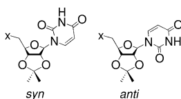
FIGURE 2 syn and anti conformations of uridine.
