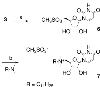
SCHEME 2 a) \text{HCl} (10%), room temperature, 12 hours; b) 65°C, 1 week.
