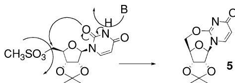
FIGURE 1 Uridine intramolecular cyclization process.
