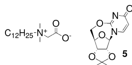
FIGURE 3 The cyclization product and the carboxy-betaine obtained refluxing 5'- O -chloroacetyl-2',3'-isopropylidene uridine and dimethyldodecylamine.
