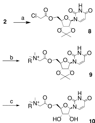
SCHEME 3 a) Chloroacetyl chloride, Py, -10^{\circ}\text{C} , 2 hours; b) dimethyldodecylamine ( \text{R} = \text{C}_{12}\text{H}_{25} ), 40^{\circ}\text{C} , 24 hours; c) DOWEX monosphere 650L resin, room temperature, 12 hours.
