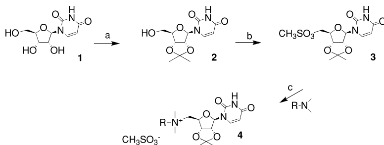
SCHEME 1 a) p-toluenesulphonic acid, 2,2-dimethoxypropane, room temperature, 1.5 hours; b) \text{CH}_3\text{SO}_2\text{Cl} , TEA, 0^\circ\text{C} , 16 hours; c) \text{R} = \text{C}_{12}\text{H}_{25} , reflux, 24 hours.
